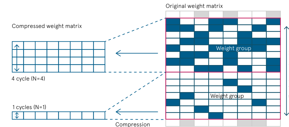
Figure 4: Compression of a Pruned Model Using DRP-AI3
