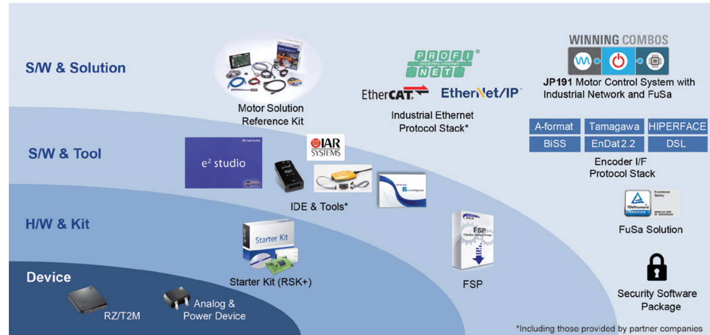
Figure 2: Development environment
