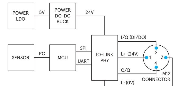
Figure 2. Building Blocks of an IO-Link Sensor
